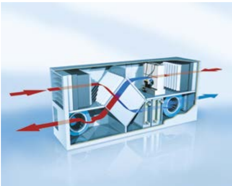
Indirect evaporative cooling with Condaire ME
