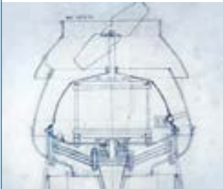
Defensor rotary atomizer from 1948
