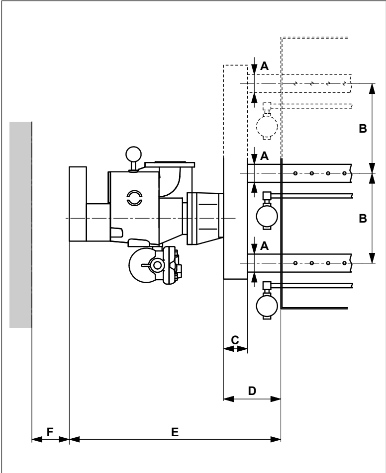
Dimensions for multiple piping
